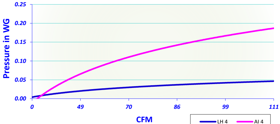
LH & AI 4 Inch Pressure Drop Test
