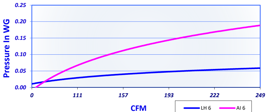
LH & AI 6 Inch Pressure Drop Test
