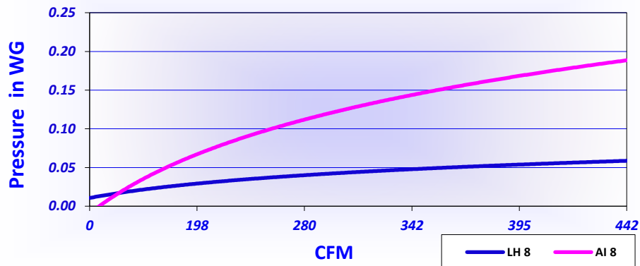
LH & AI 8 Inch Pressure Drop Test
